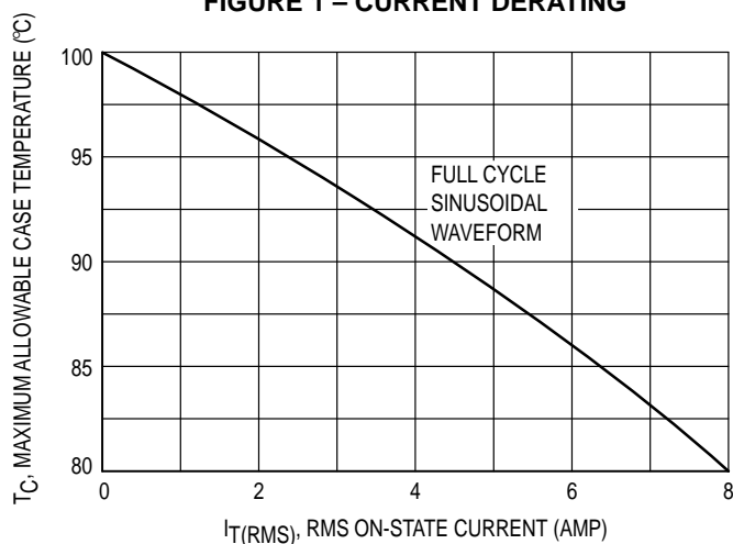
FIGURE 1 – CURRENT DERATING
